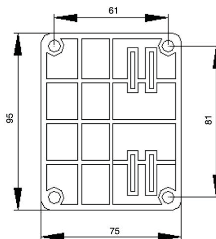
MOUNTING BRACKET
